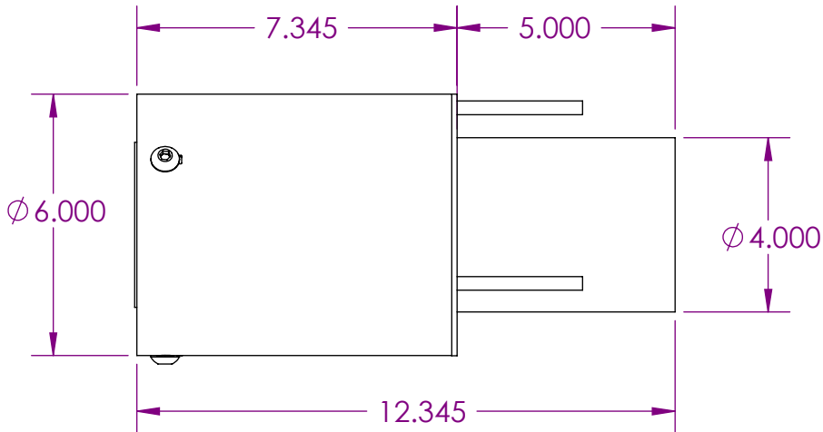
EXPANDED POSITION
